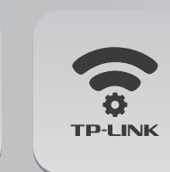
Tether APP
